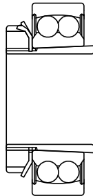
Bearing with adapter sleeve
