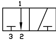
3 PORT 2 POSITION
