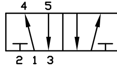
5 PORT 2 POSITION
