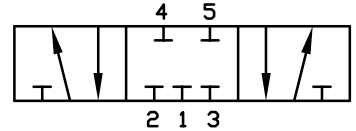
5 PORT 3 POSITION
