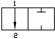
2 PORT 2 POSITION
